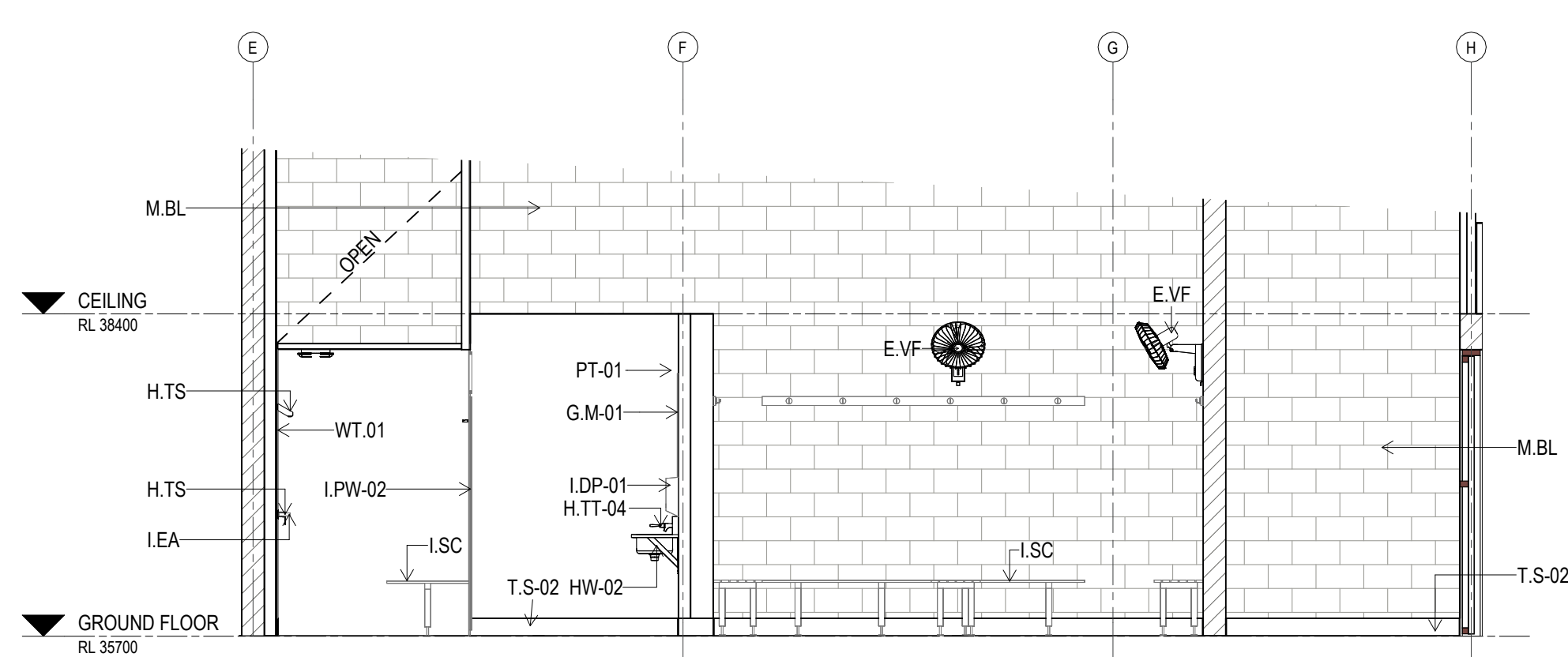
A ELEVATION CHANGE ROOM 1 Scale: 1 : 50
