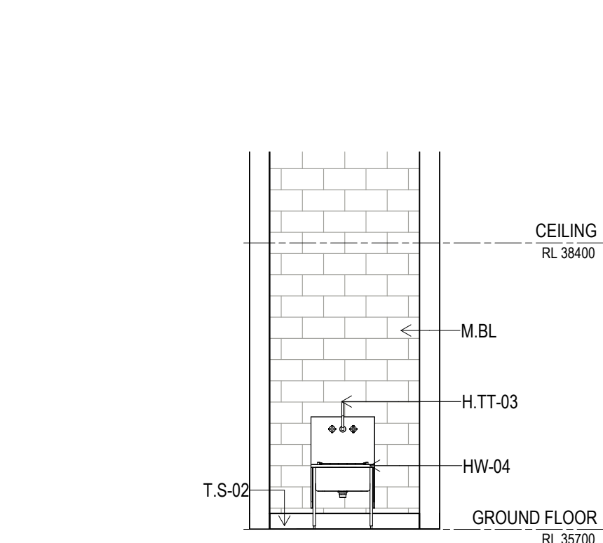
6 ELEVATION CLEANERS Scale: 1 : 50
