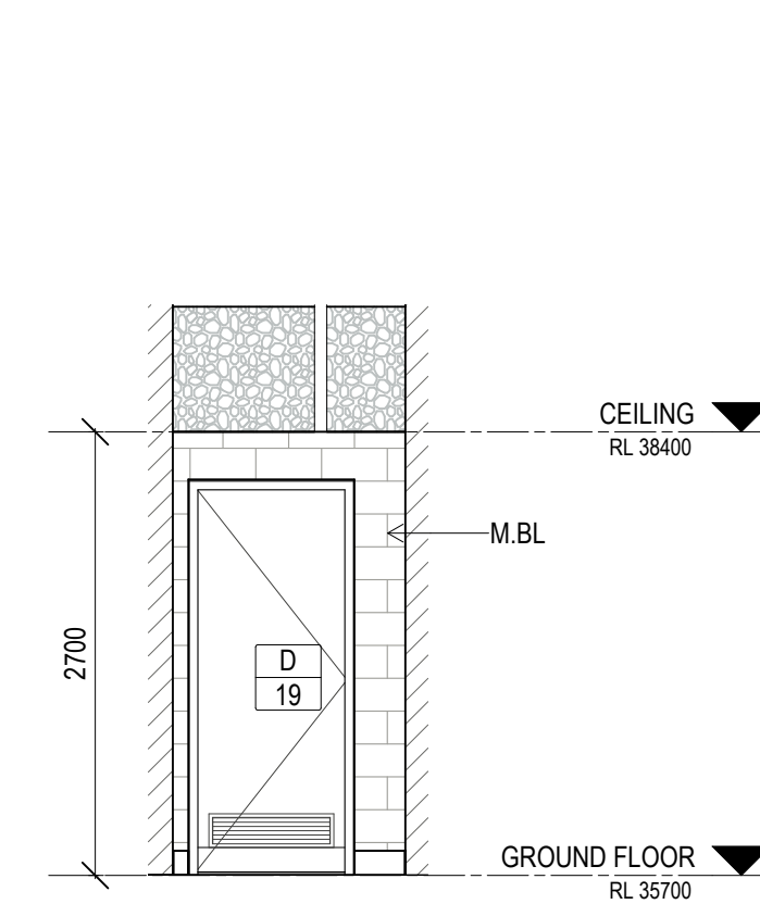
4 ELEVATION CLEANERS Scale: 1 : 50
