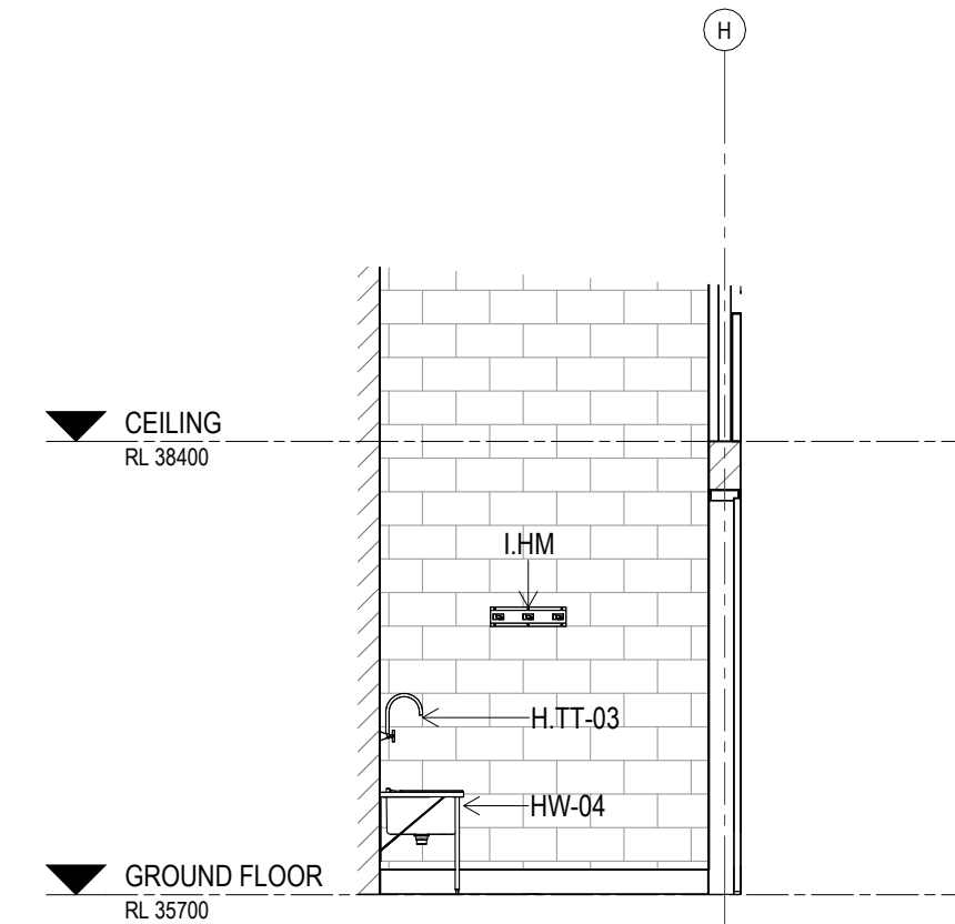
3 ELEVATION CLEANERS Scale: 1 : 50
