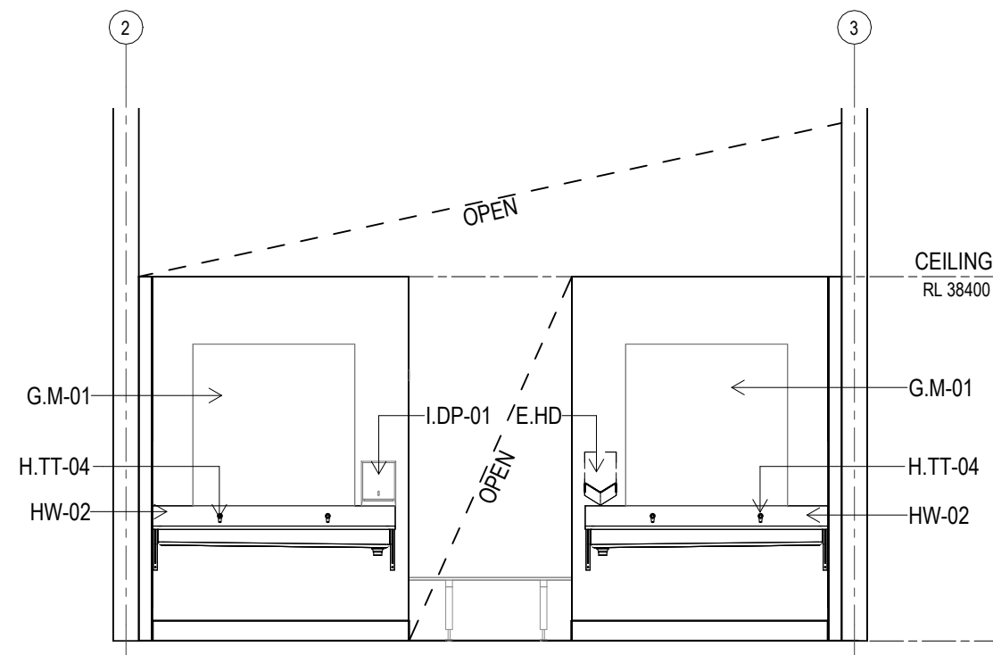
H ELEVATION CHANGE ROOM 1 Scale: 1 : 50
