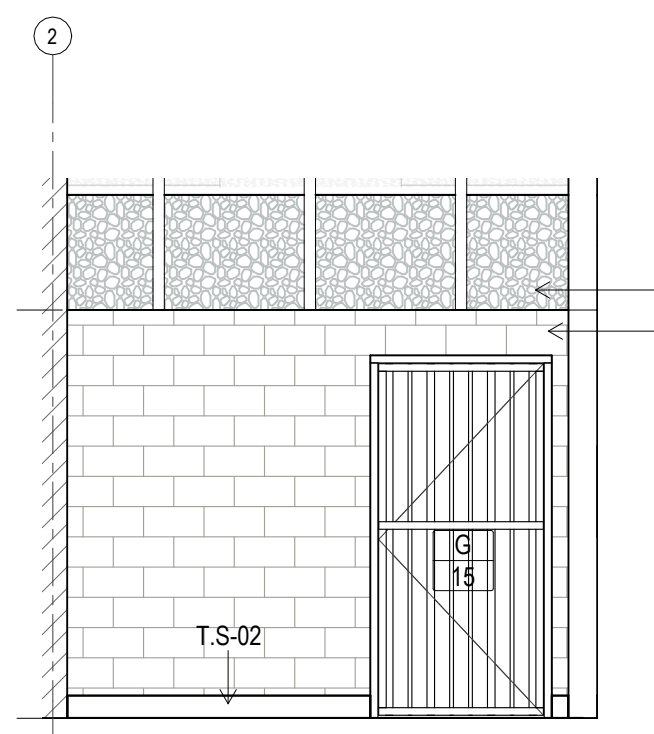
G ELEVATION CHANGE ROOM 1 Scale: 1 : 50
