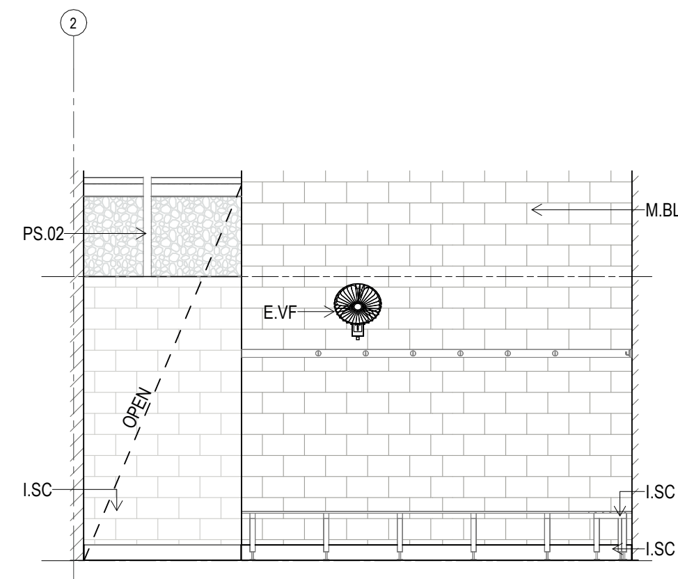
B ELEVATION CHANGE ROOM 1 Scale: 1 : 50
