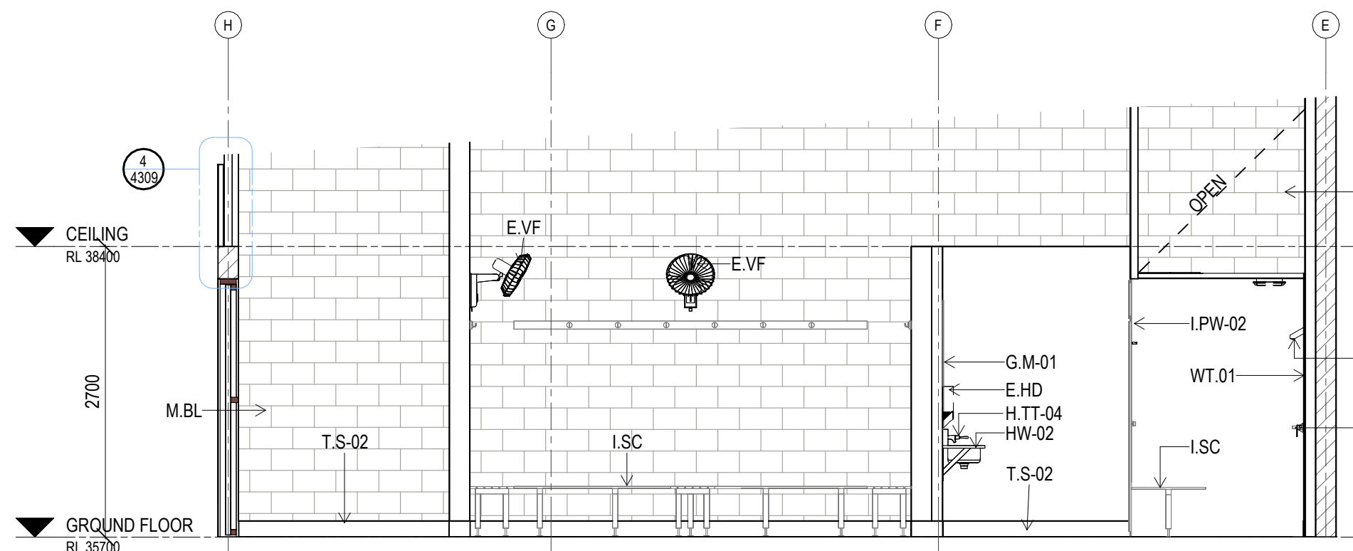
C ELEVATION CHANGE ROOM 1 Scale: 1 : 50
