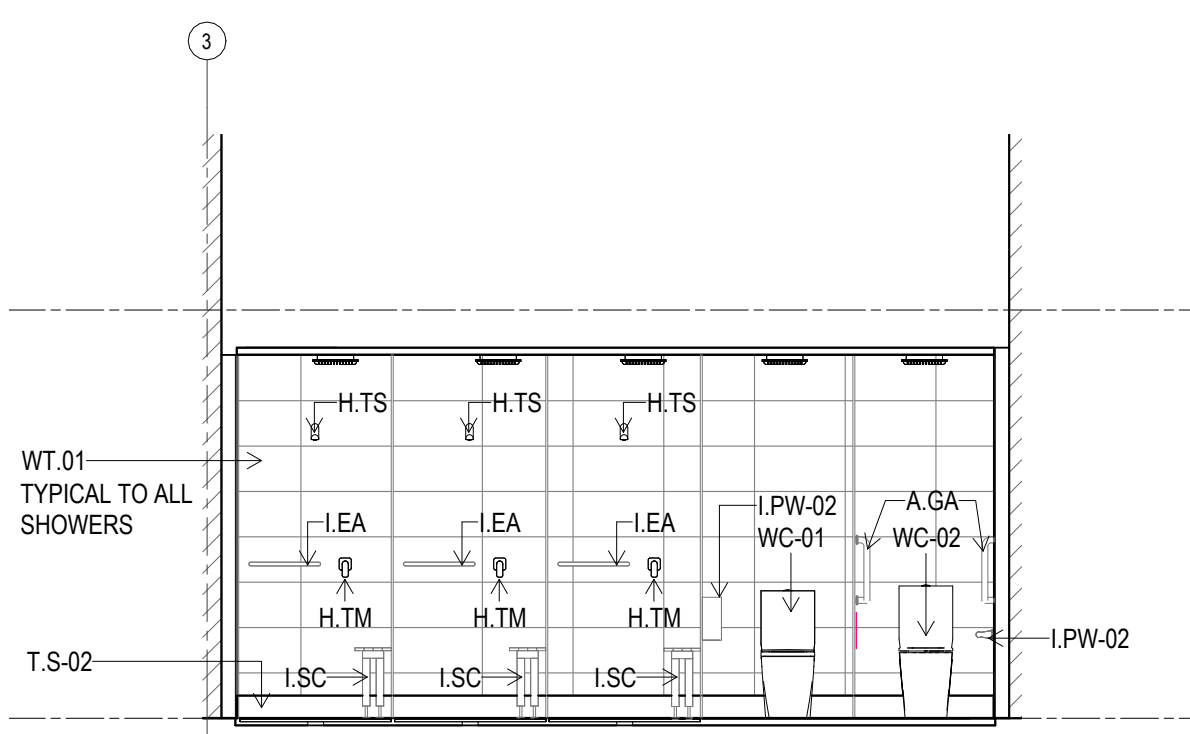
F ELEVATION CHANGE ROOM 1 Scale: 1 : 50
