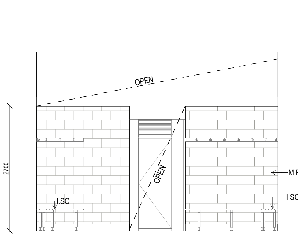
D ELEVATION CHANGE ROOM 1 Scale: 1 : 50
