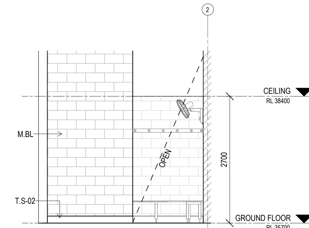
I ELEVATION CHANGE ROOM 1 Scale: 1 : 50
